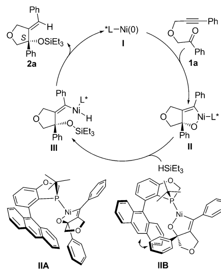
Figure 4. Proposed mechanism and stereochemical model for the asymmetric reductive cyclization of alkynones. \text{L}^* = (S)\text{-AntPhos} .
